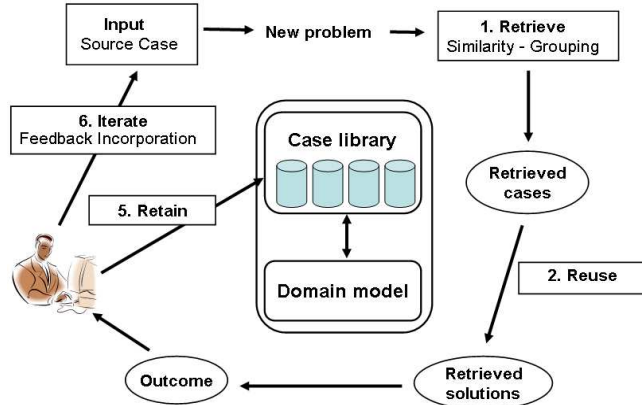
Fig. 7. DieToRecs - Seeking for Inspiration technique
