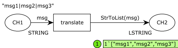
Fig. 21. Message translator in CPN tools.
