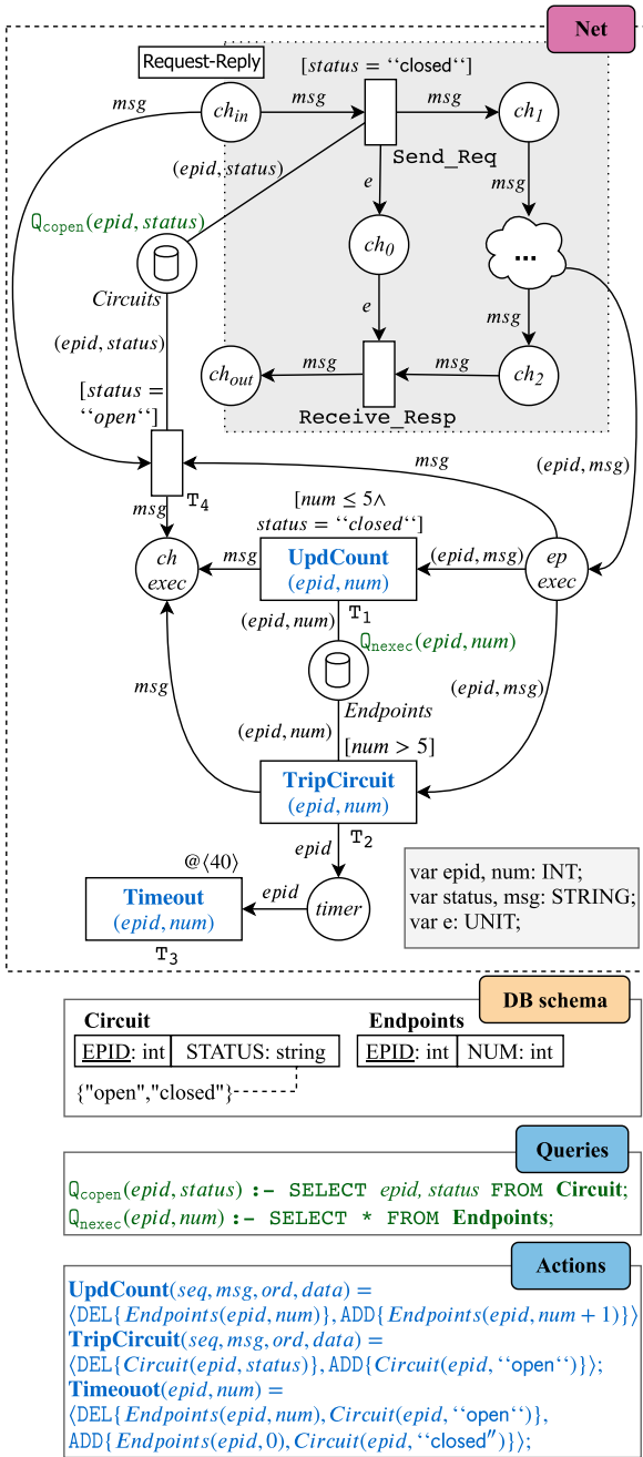
Fig. 12. Circuit breaker realization in timed db-net.
