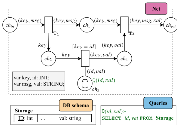
Fig. 10. Content enricher realization in timed db-net.
