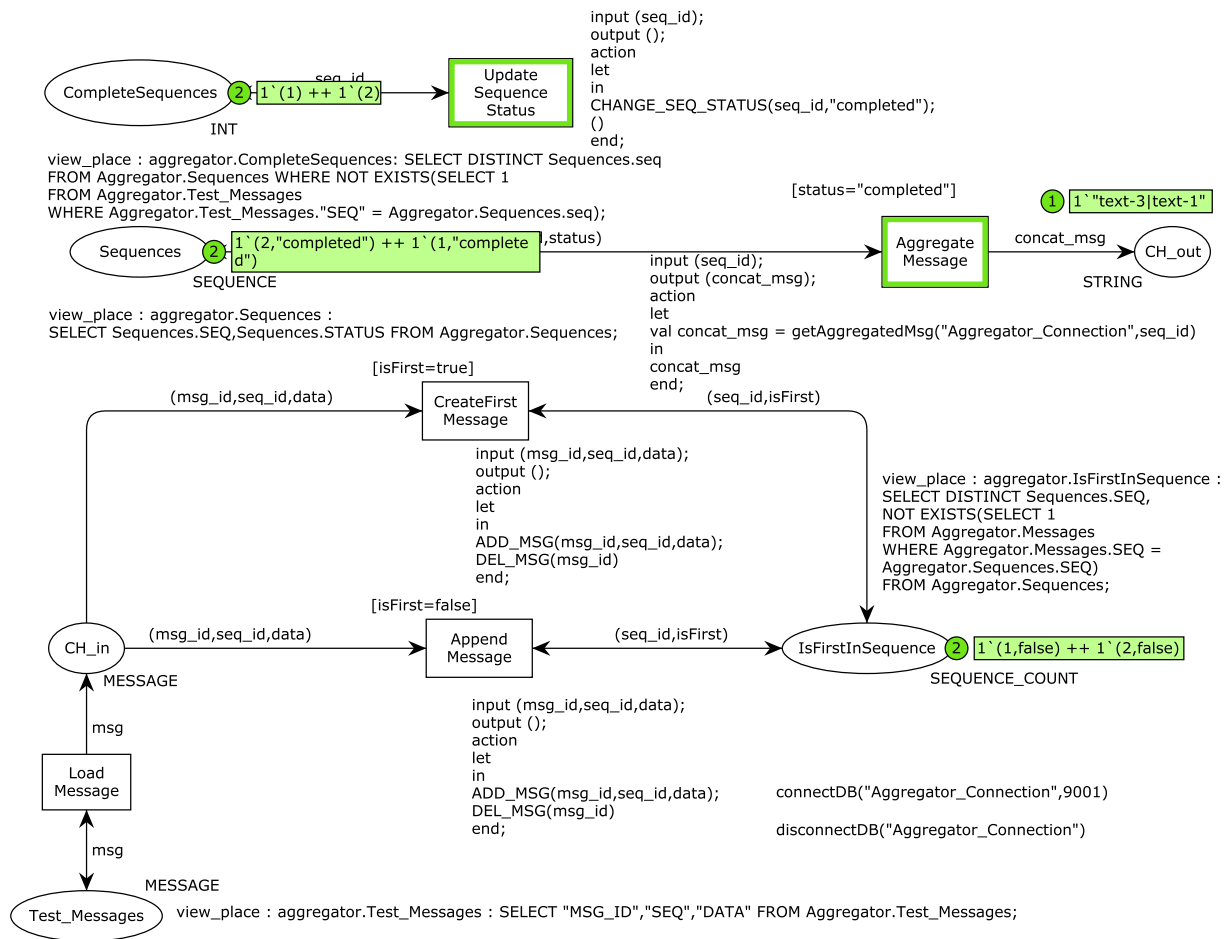
Fig. 24. Aggregator in CPN tools.
