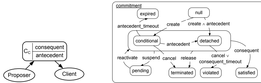
Fig. 4. Commitment notation (left) and lifecycle (right). [?]
