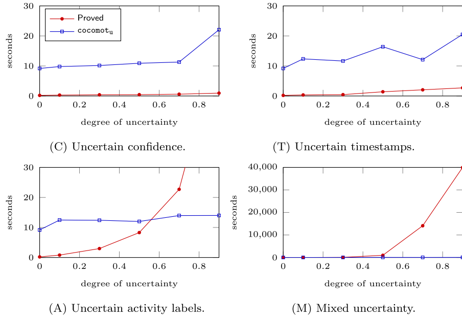
Fig. 3. Comparison of cocomot u (best-realization cost) and Proved .
