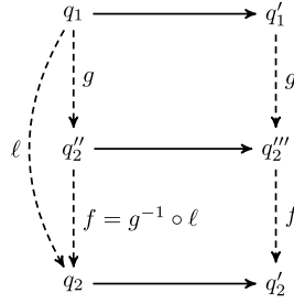
Fig. 2. Relationships among the states q_1, q_1', q_2, q_2', q_2'', q_2''' involved in the proof of Theorem 7.
