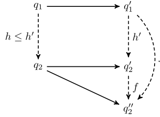
Fig. 4. Relationships among the states q_1, q_1', q_2, q_2' involved in the proof of Lemma 14.
