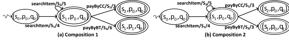
Fig. 3. Two possible composition of services \mathcal{S}_1 , \mathcal{S}_2 , and \mathcal{S}_3 for the target service \mathcal{S}_t in Fig. 1(c)
