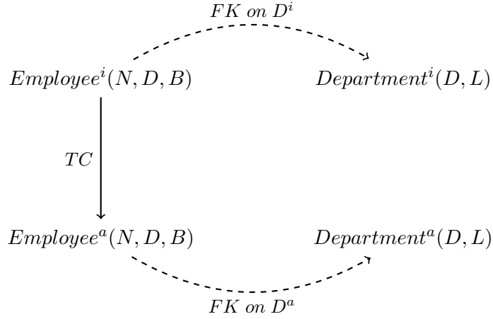
Figure 5.1: Visualization of reasoning example with FK
