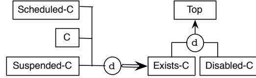
Fig. 2. EER graphical rendering of the \mathcal{DLR}_{US} axioms for status classes; Top represents the universe of discourse, arrow denotes subtype, and the encircled d means disjoint (Source: [5]).
