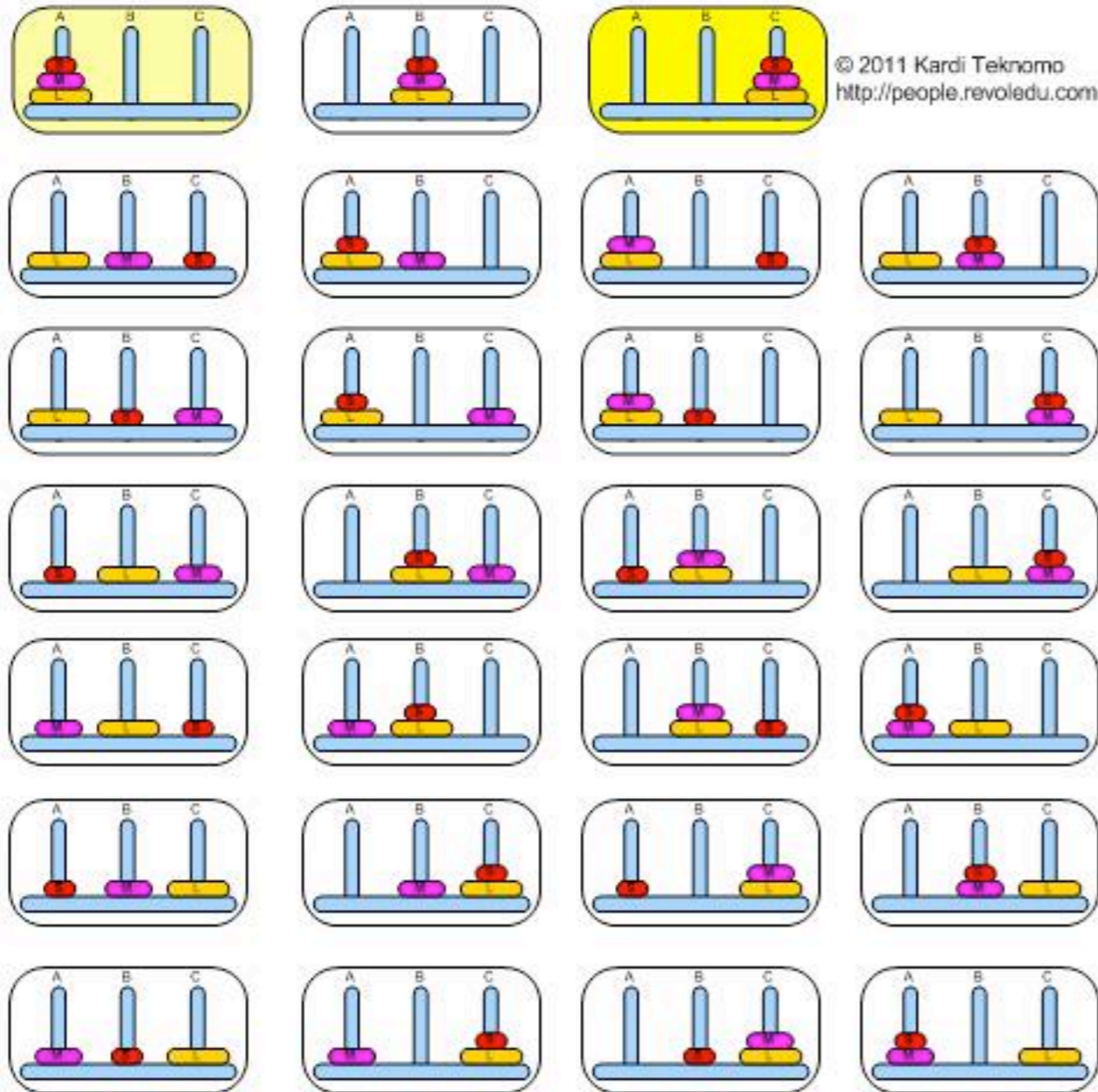
All Possible States of Tower of Hanoi
