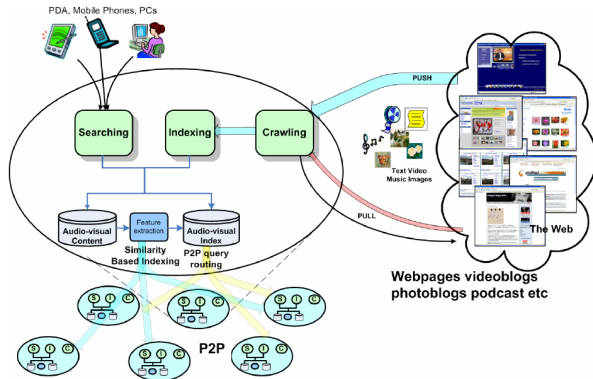
Figure 1. SAPIR components and functions
