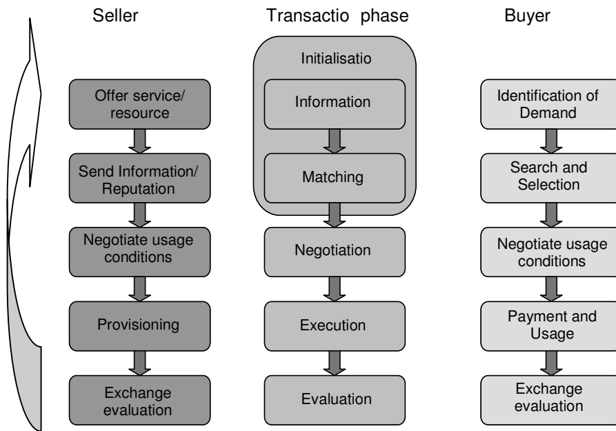
Figure 2: Lifecycle of Agents
