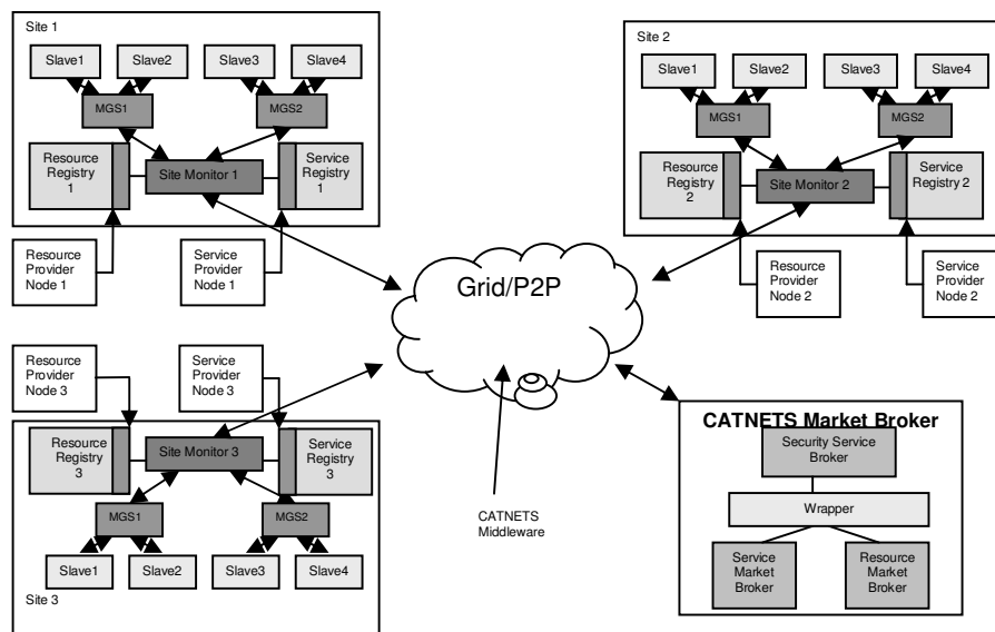
Figure 5: The Proposed Multiagent System Architecture for Indexing and Querying
