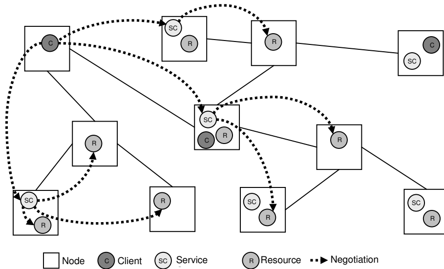
Figure 3: Catalactic middleware as a network of agents
