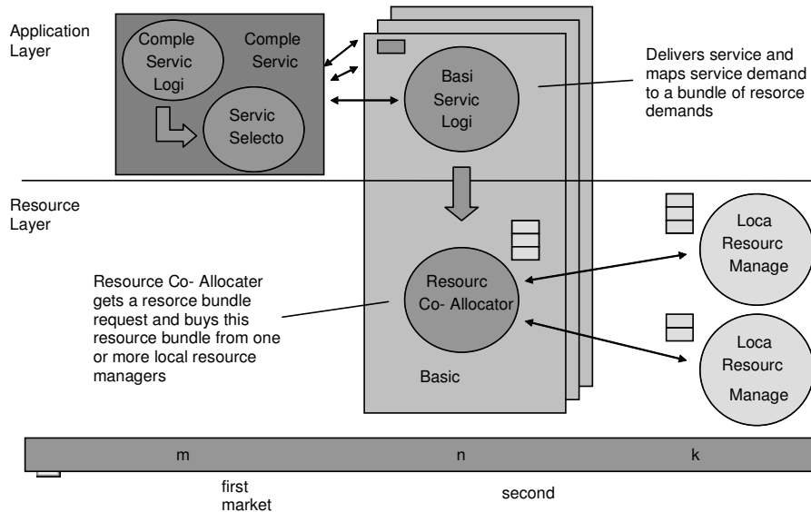
Figure 1: Catalaxy-based Grid Market Model
