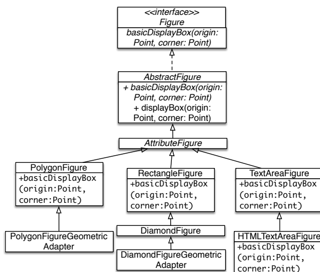
Fig. 1: Sample class hierarchy from JHotDraw, with multiple implementations of the operation basicDisplayBox(Point, Point) .
