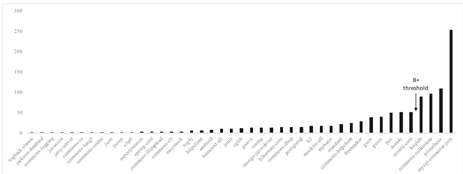
Fig. 11 Frequency of breaking features, excluding APIs that never directly introducing breaking changes
