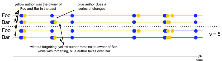
Fig. 7 Example of Syde ownership map
