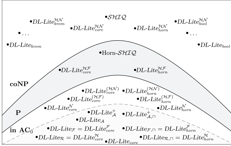
Figure 3: The DL-Lite family and relations.
