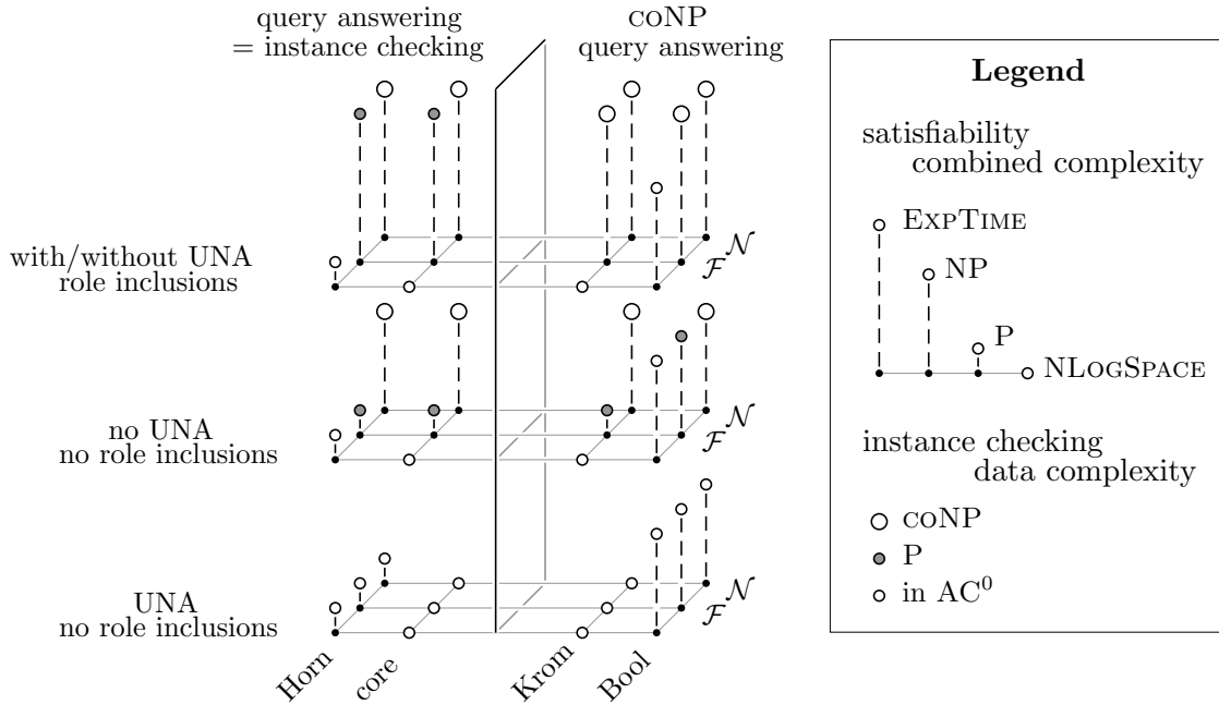
Figure 6: Complexity of basic DL-Lite logics.
