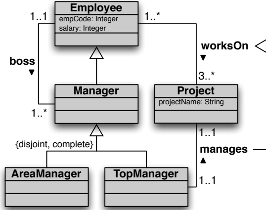
Figure 2: A UML class diagram.
