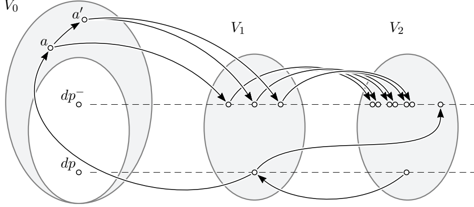
Figure 4: Unraveling model \mathfrak{M} (first three steps).
