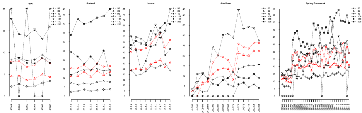
Figure 10: Z-score plots of motifs over releases of the SUTs. Red lines indicate the most simple types.
