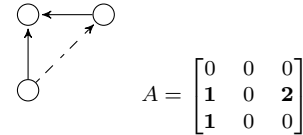
Figure 5: Coloured motif - Proxy pattern
