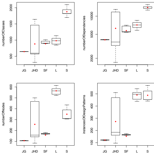
Figure 7: From top left clockwise: number of classes, links between classes, design pattern instances, and nodes.
