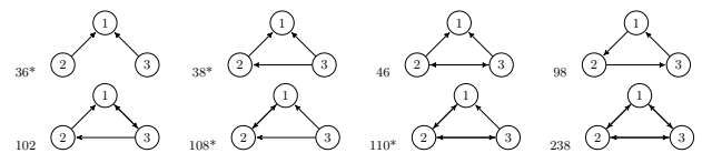
Figure 9: Topology of the motifs appearing in at least one release of one SUT. Motifs labelled with * appear in all releases of all systems.
