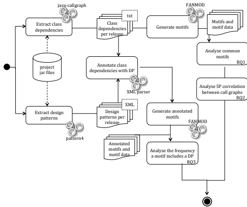
Figure 6: Activity flow of the analysis
