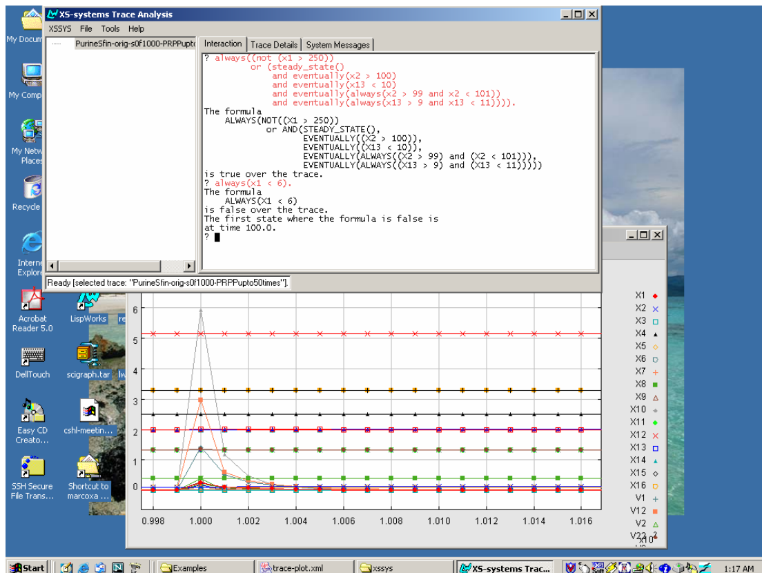
Figure 10. The in silico trace of the “final model” from [4]. We arbitrarily increased the level of PRPP (variable X1) to more than 250 at time step 100. The XSSYS system correctly answers both queries. Because of numerical fluctuations we had to ask a less stringent question about the steady state value of IMP (variable X2) and HX (variable X13).
