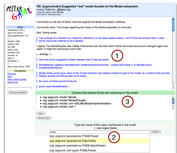
Figure 3. Web Application: E-Mail annotation
