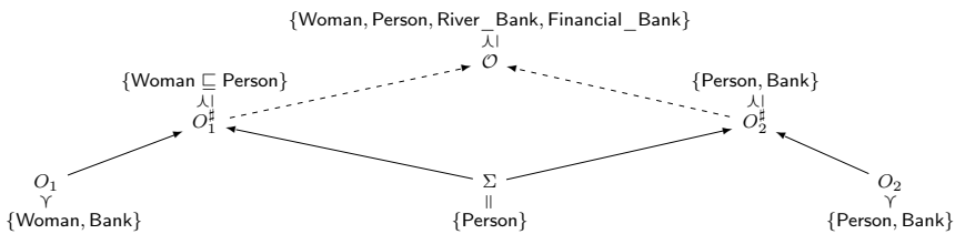
FIGURE 8. M-alignment: integration through bridge along extensions
