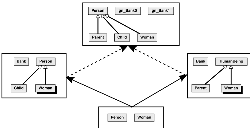
FIGURE 23. Colimit of a V-alignment in HETS.
