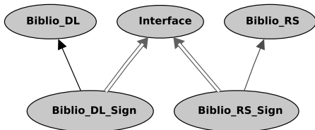
FIGURE 24. W -alignment in HETS.
