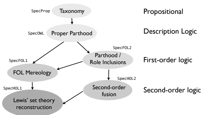
FIGURE 17. Heterogeneous specification of mereology
