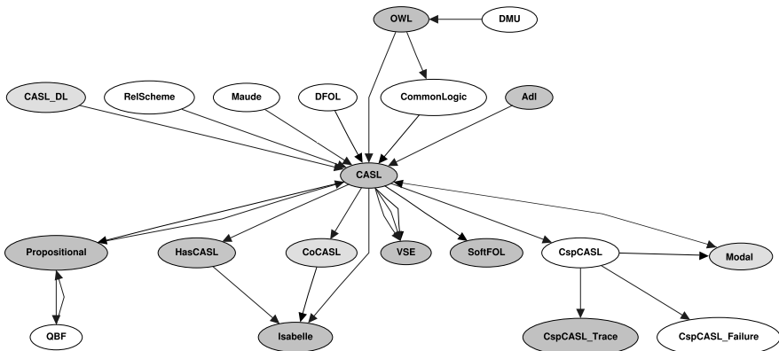
FIGURE 13. HETS' logic graph
